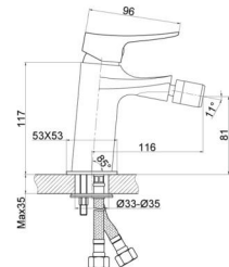
■ SH570-02 Single handle bidet mixer Φ35
