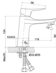
■ SH570-01 Single handle basin mixer Φ35
