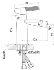
SH571-02 Single handle bidet mixer Φ35
