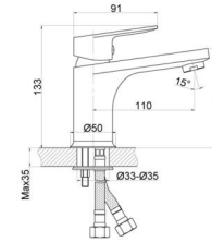
SH567-01 Single handle basin mixer Φ35
