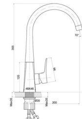
■ SH570-09 Single handle bath mixer Φ35
